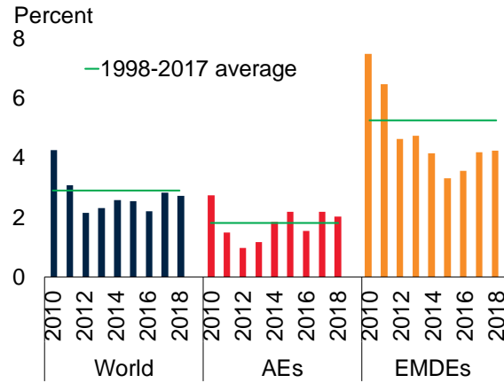
Figure 1. Global Growth
