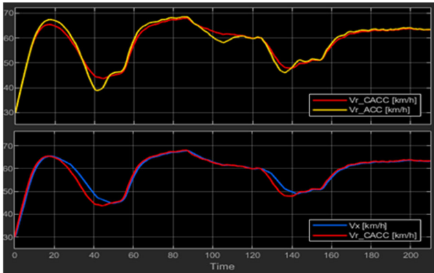
Fig. 9 Comparison between ACC/C-ACC references and vehicle speed
